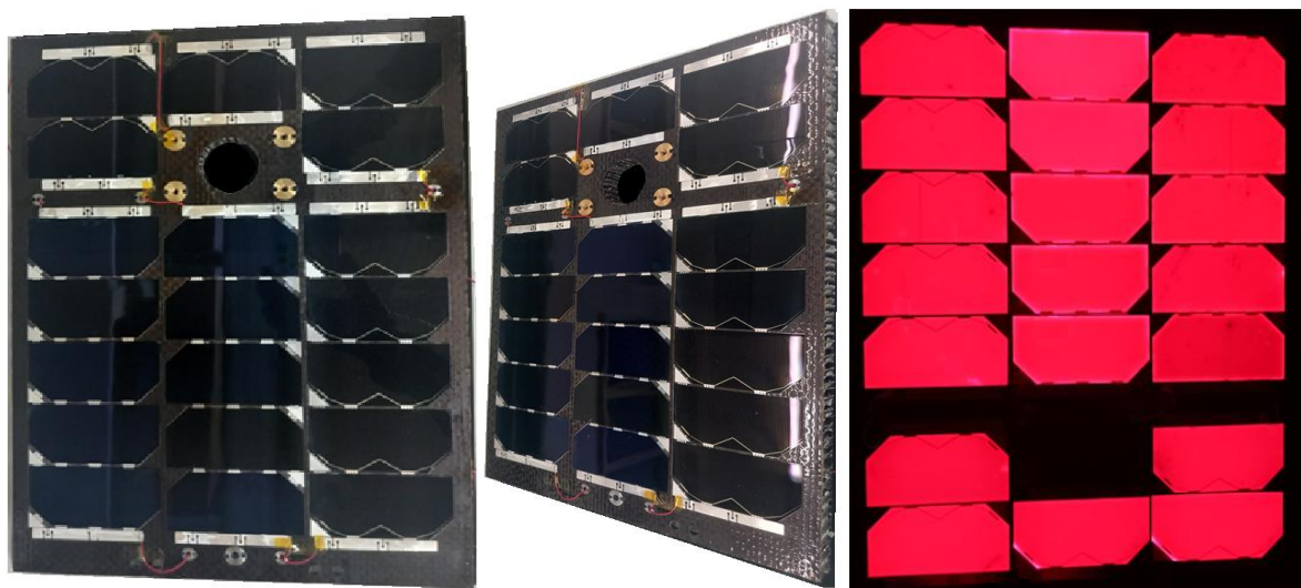
Example of the solar array for mini or small satellite
